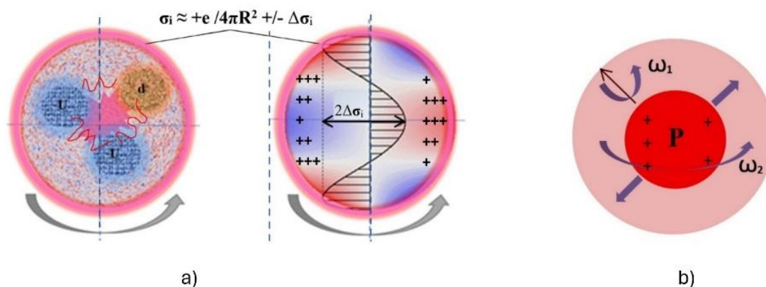
Figure 1: Interactions of Quarks U and d in the Proton Structure Led to a Periodic Change in the Charge Density \Delta\sigma_i on the Proton Surface and a Change in the External Electric Field Strength \Delta E , Respectively (a) and Oscillatory and Rotational Motions of the Proton in the Nucleus Lead to Additional Fluctuations of the Electric Field E of the Proton (b)
