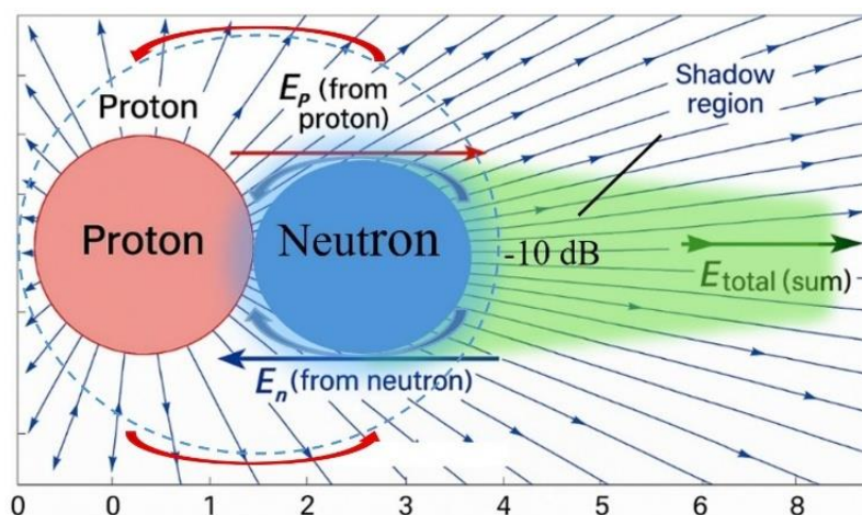
Figure 4: General Diagram of the Formation of a Low-Potential Channel in the Coulomb Field of the Nucleus (Shadow Region) Due to the Influence of a Neutron
