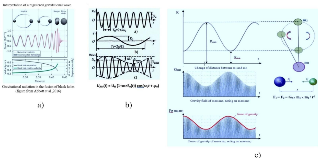
Figure 10: Structure of Gravitational Waves
