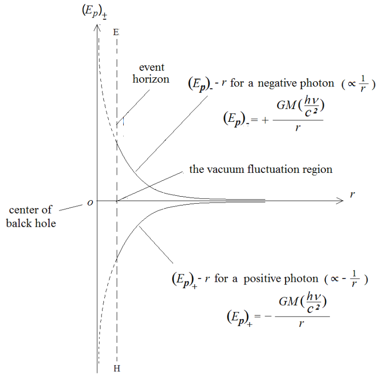
Figure 5: The Relations of The Gravitational Energies of The Positive or Negative Photon E_{p+} and E_{p-} to the Distance r from the Photons to the Center of The Black Hole
