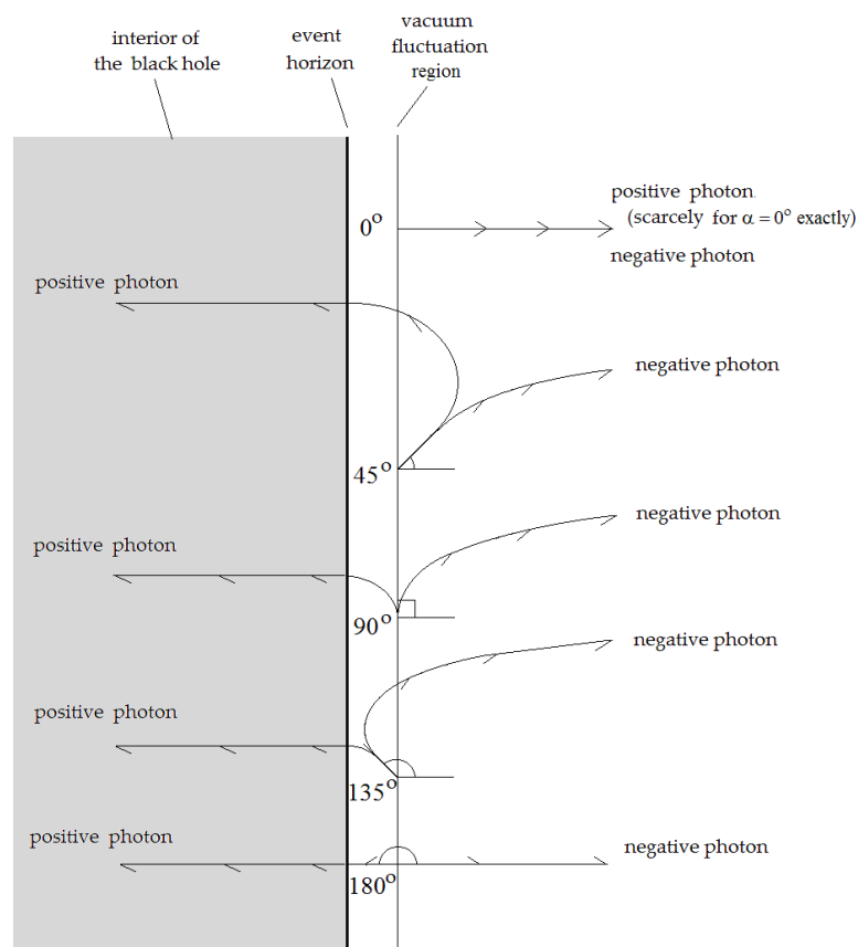
Figure 6: The Extremely Powerful Gravitational Field Near the Event Horizon Promotes the Virtual Pairs of Positive and Negative Particles to Separate, Going Forward Along Different Ways. Almost all the Positive Photons Enter the Black Hole and Combine with the Main Mass of the Black Hole. All the Negative Photons are Repelled to the Cosmic Space, Annihilate with the Matched Photons they Encountered in their Ways
