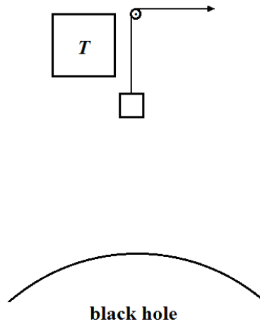
Figure 7: Geroch and Bekenstein's Gravitational Engine
