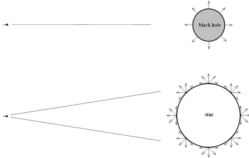
Figure 3: Two Far-Left Observers
