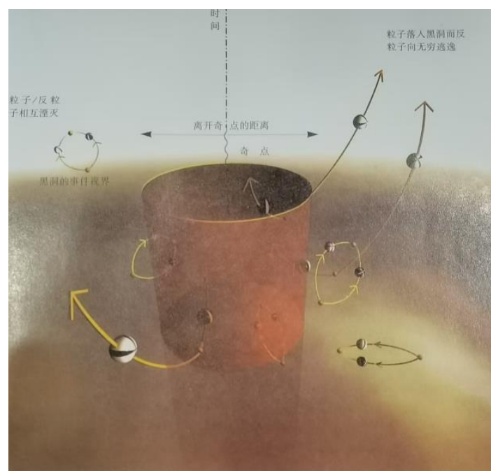
Figure 4: Hawking's Picture Shows that the Initial Directions of the Velocities of the Photon and anti Photon Produced in a Vacuum Fluctuation are Identical, and May be in any Direction in the 4\pi Solid Angle. He is Correct. (This Picture is Quoted from Hawking's A Brief History of Time.)
