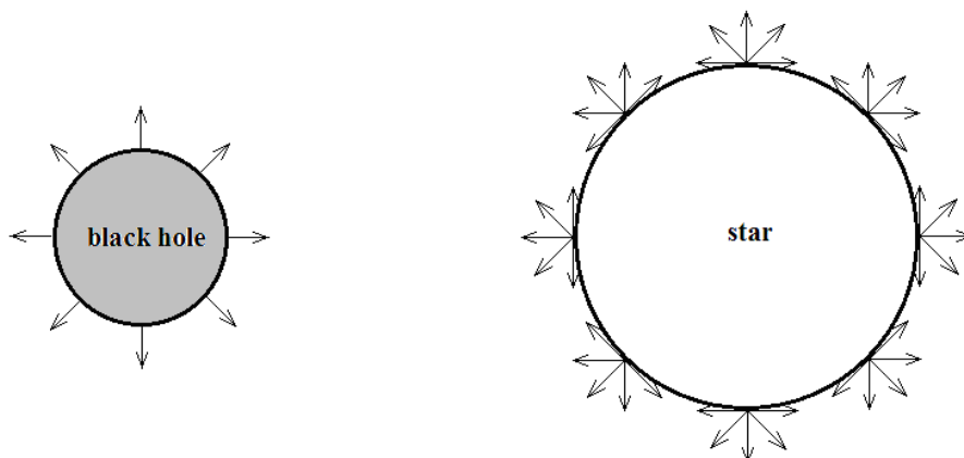
(a) the Hawking radiation of a black hole
