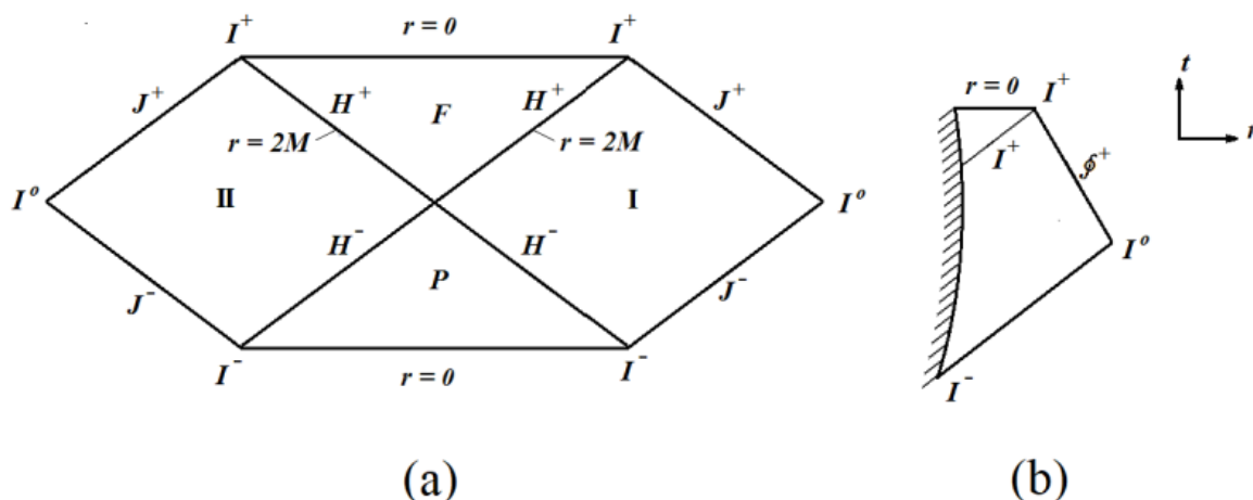
Figure 1: Derivation of Hawking's Thermal Radiation
