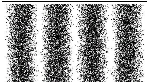
Figure 2: The Photosensitive Results of Electrons Passing Through the Double Slit One by One. After a Photon Passes Through the Double Slit, Hitting the Receiving Screen Is Just A Small Bright Spot. It is Not Convenient to Explain It Using the Term 'Discrete Wave Screen Photosensitive Reaction'
