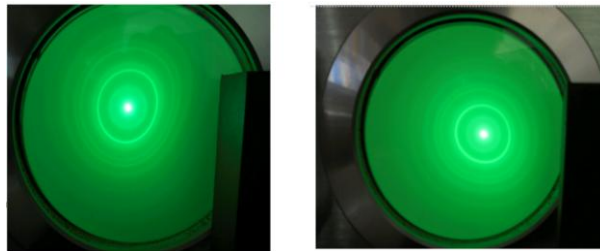
Figure 3: The Result of Using Magnetic Field to Interfere with Electron Diffraction. The Electron Beam Moves Laterally Along the Direction of Force, Causing Diffraction Fringes to Deform and Move as A Whole, But Not Disappear. During the Diffraction Process, Electron Rays Can Exhibit Both Particle Characteristics and Wave Law Simultaneously
