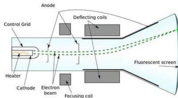
Figure 4: Schematic Diagram of Thomson Cathode Ray Deflection Experiment Principle Image Source: https://p0.ssl.qhimgs1.com/sdr/400___/t0136f39cb9fcded8d0.jpg
