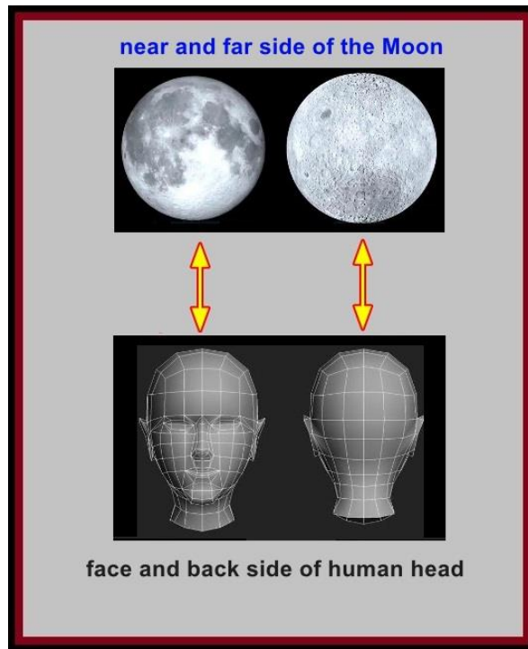
Figure 6: The One-To-One Correspondence of The Outline Between the Moon and Human Head
