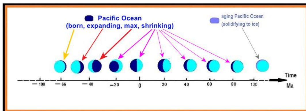
Figure 9: The Evolution Phase of The Pacific Ocean
