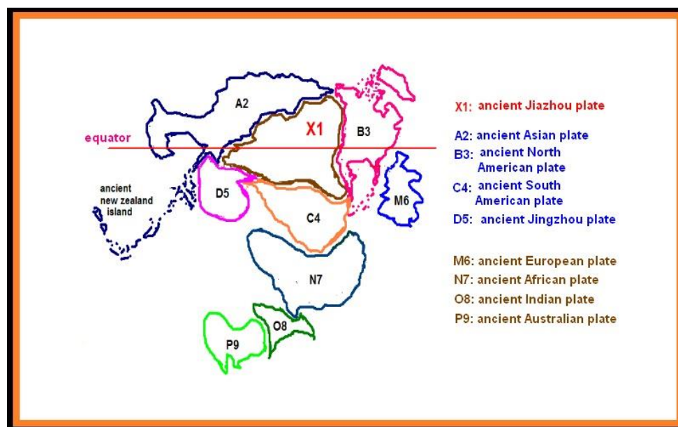
Figure 8: The Jigsaw Recover of The Unique Supercontinent of The Earth 66 Ma Ago
