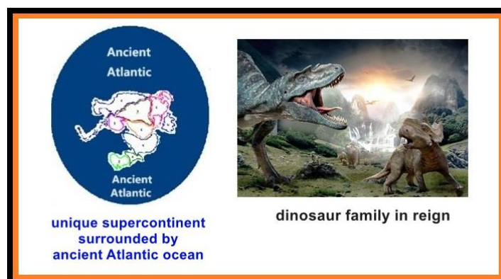
Figure 18: The Reign Termination of The Dinosaur Family on The Unique Supercontinent 66 Ma Ago
