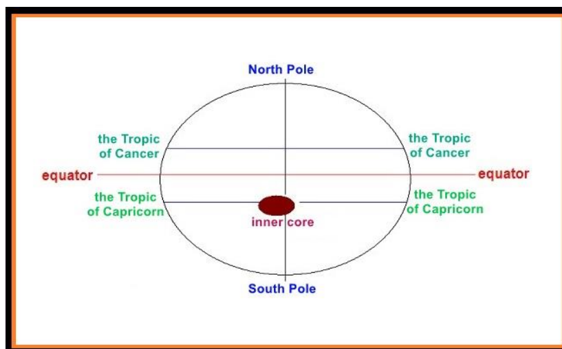
Figure 23: The Location of The Earth's Inner Core
