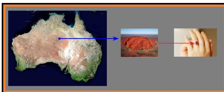
Figure 25: The Celestial Body Ring, The Ayers Rock, That Located in The Geometrical Center of The Main Island of Australia
