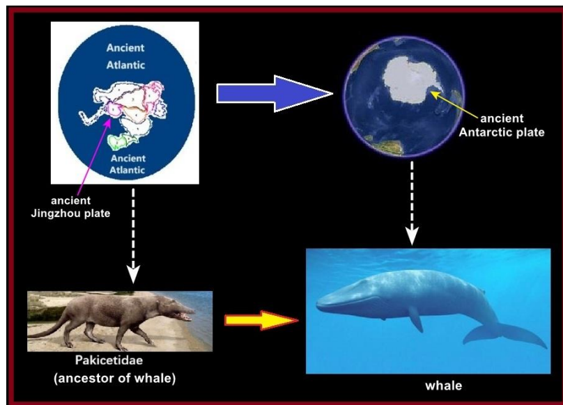
Figure 19: Case Evolution of Pakicetidae to Whales in The Past 66 Ma Base on The Dissembling of The Unique Supercontinent
