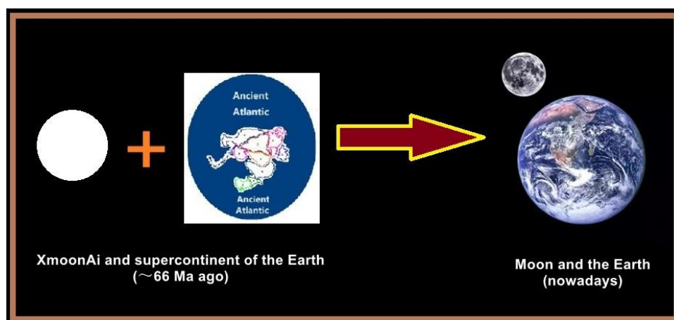
Figure 5: The Birth of The Moon
