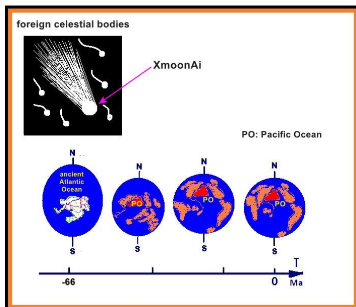
Figure 21: It Was the Xmoonai That Opened the Door of The Brilliant Highlight Scene of Anthropocene
