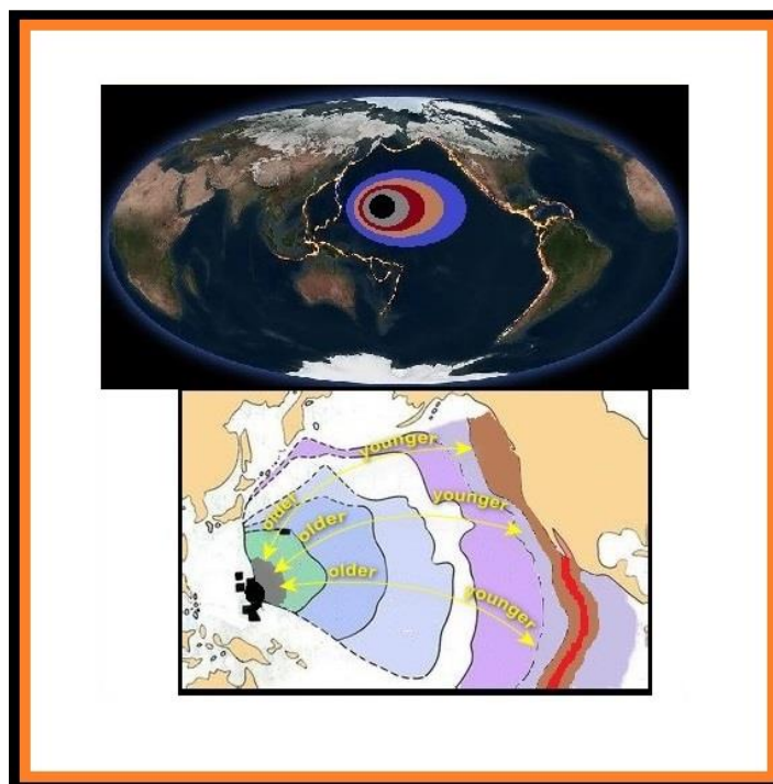
Figure 12: The Formation of Hinted Black Hole (Hbh) On the Ancient Jiazhou Plate Hidden in the Ocean Floor of Northwestern Pacific Ocean
