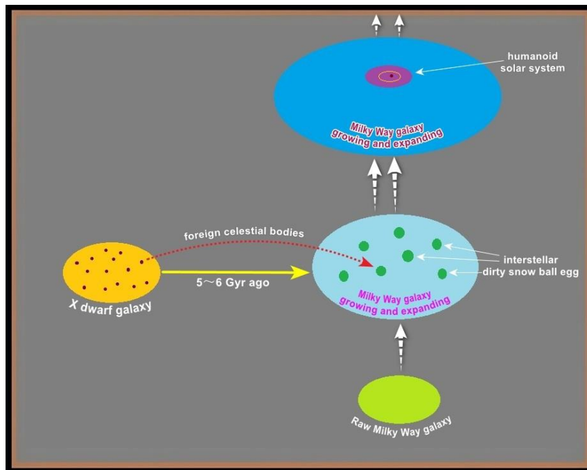
Figure 2: The Simplified Evolution Tree of The Milky Way Relating to The Origination of The Sun
