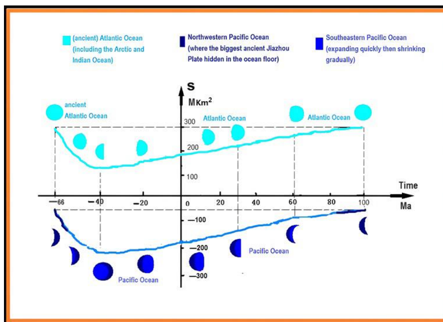
Figure 16: The Competitive Evolution Between the Pacific Ocean and the (Ancient) Atlantic Ocean
