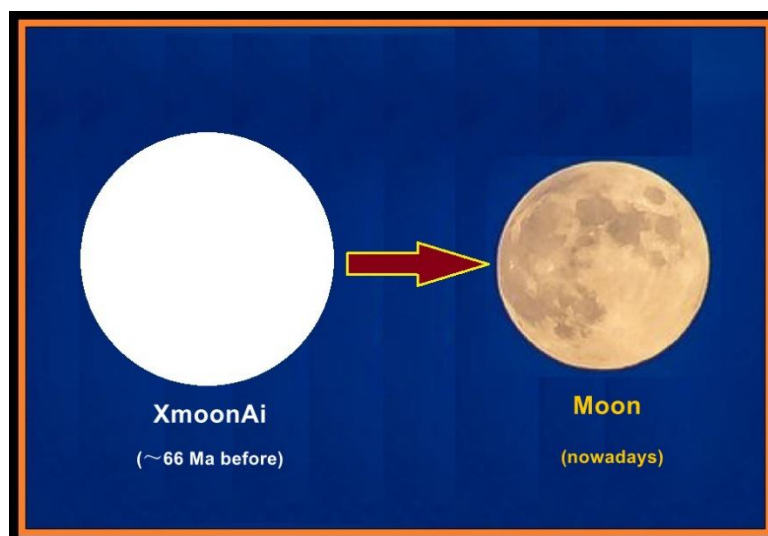
Figure 4: Xmoonai, The Predecessor of The Moon, Originated from The Xplus Dwarf Galaxy
