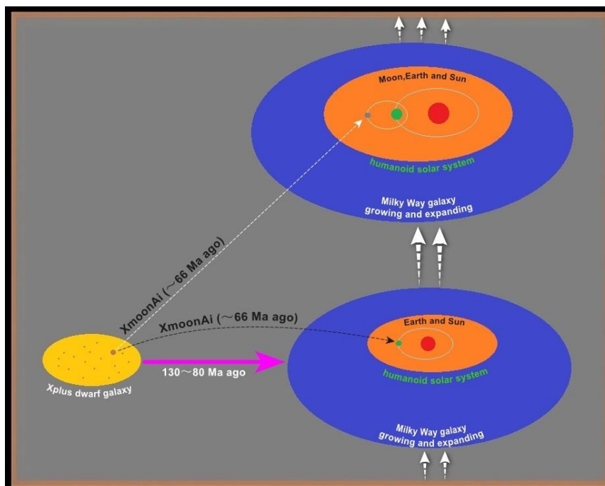
Figure 3: The Simplified Evolution Tree of The Milky Way Relating to The Origination of The Moon
