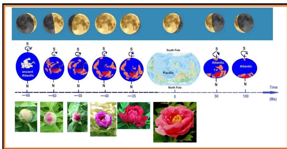
Figure 15: The Full Blooming of The Unique Supercontinent Flower on the Earth Upside Down
