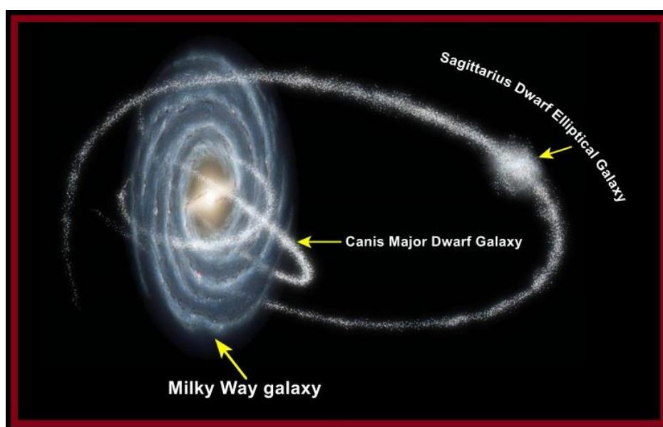
Figure 1: The Colliding and Merging Between the Milky Way Galaxy and Other Dwarf Galaxies
