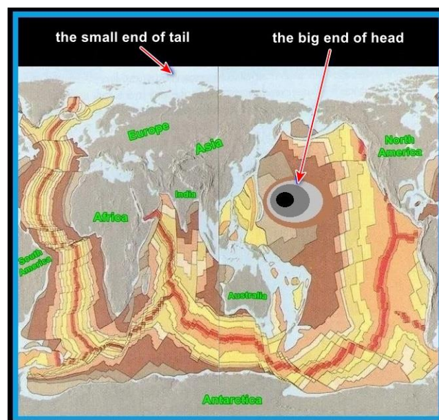
Figure 20: The Formation of the "ω" Shape Giant Dragon of Cracking Ridge on The Ocean Floor Globally
