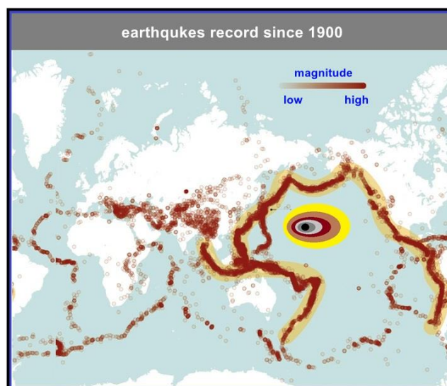
Figure 14: The Celestial Body Language Implied by the "Ω" Shape Pacific Ring of Fire
