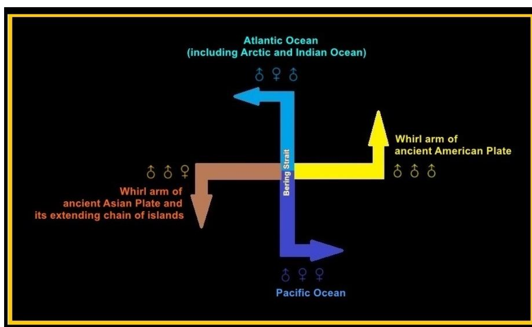
Figure 11: The Birth of The Cross “+” Shape Ocean-Plate Whirlpool of Double Whirl Arms
