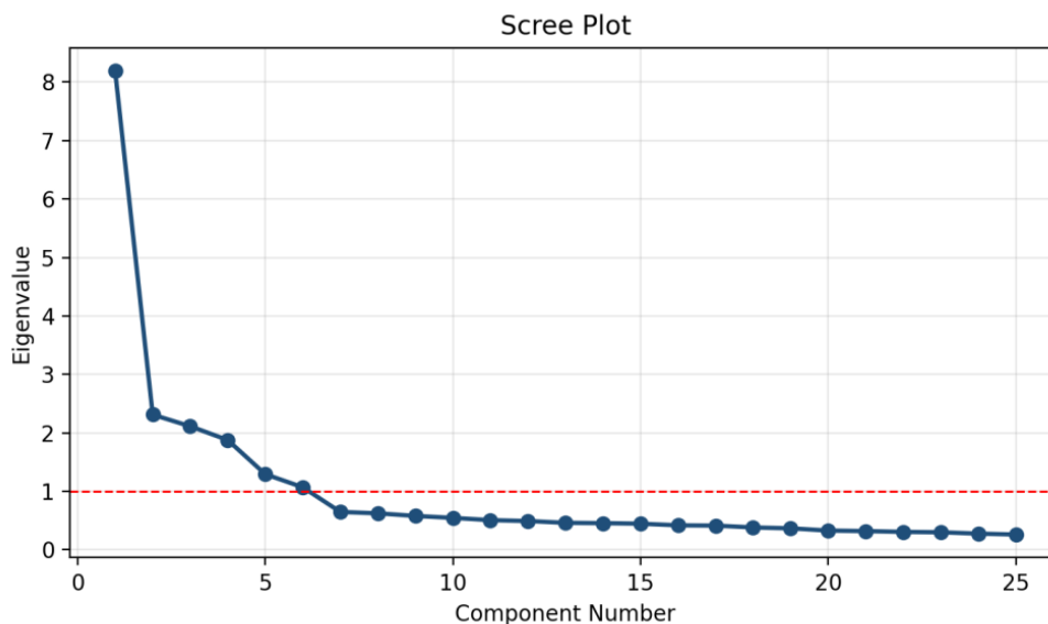
Figure 3: Scree Plot of Eigenvalues
