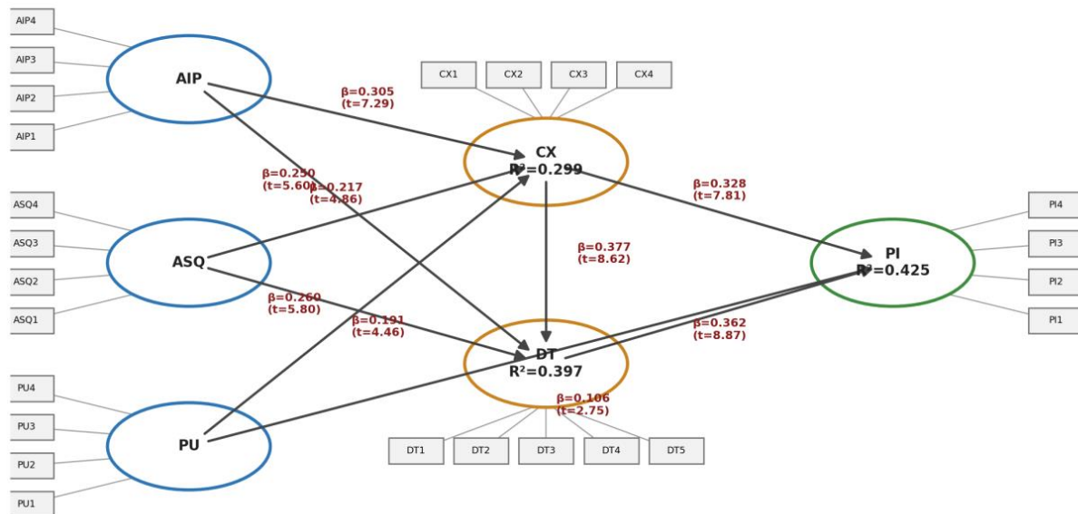
Figure 4: Structural Model Results with Path Coefficients and t-values
